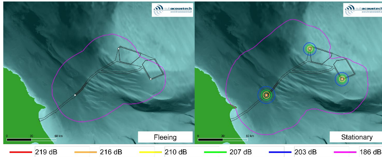
Figure 5-5 Contour plots showing the in-combination impacts of concurrent installation of multi-leg foundations at three locations across DBS for fish using the pile driving Popper et al. (2014) criteria assuming both a fleeing and stationary animal
