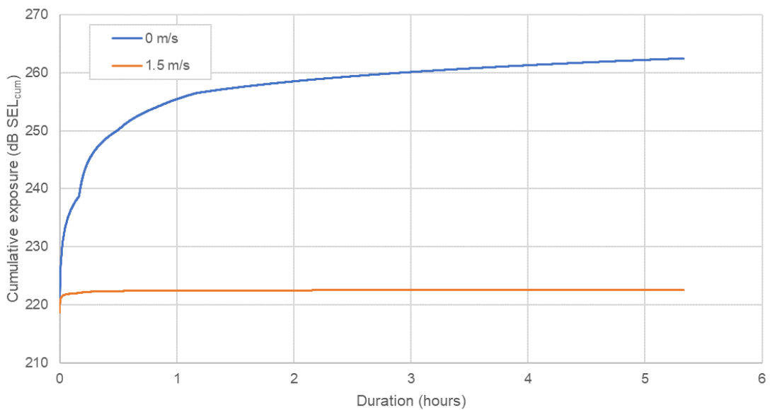
Figure 4-4 Cumulative received noise levels ( SEL_{cum} ) for receptors during monopile foundation parameters at the Dogger Bank West: West location, assuming both a stationary and fleeing receptor starting at a location 1 m from the noise source
