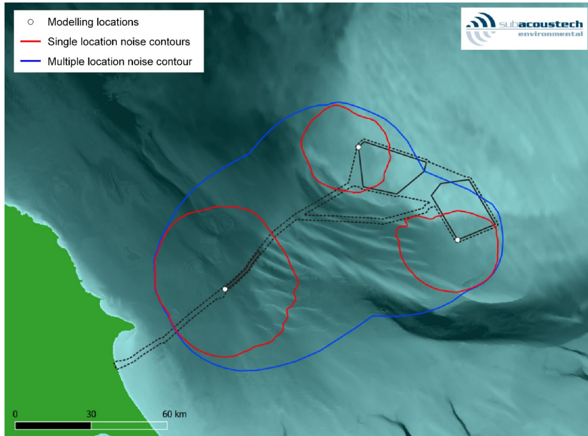
Figure 5-1 Example contour plot showing the interaction between three noise sources when occurring simultaneously (TTS in fish, 186 dB SEL_{cum} , fleeing animal)
