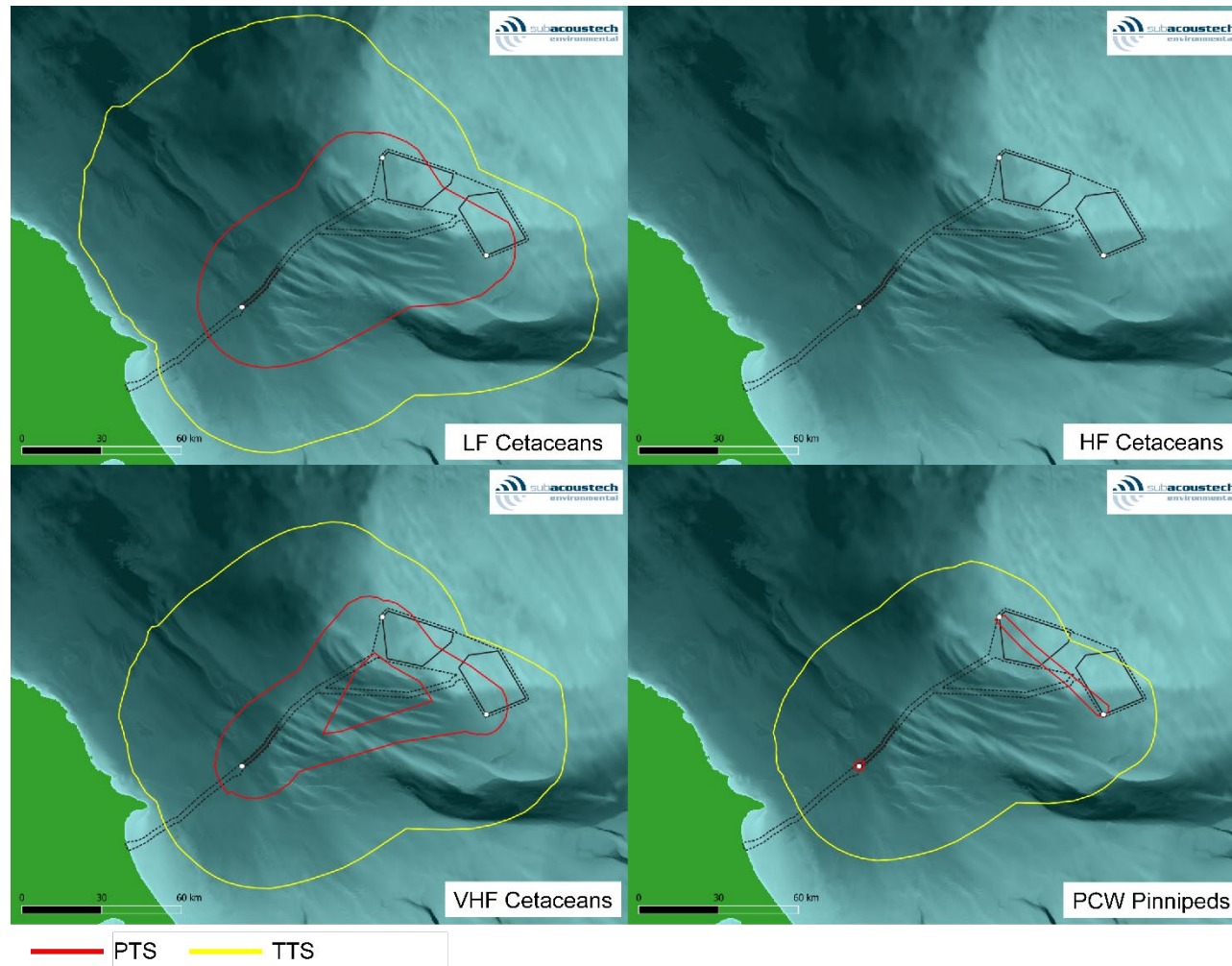
Figure 5-4 Contour plots showing the in-combination impacts of concurrent installation of multi-leg foundations at three locations across DBS for marine mammals using the impulsive Southall et al. (2019) criteria assuming a fleeing animal
