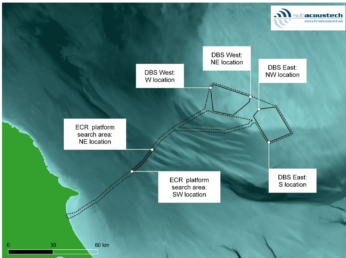
Figure 4-2 Approximate positions of the modelling locations at DBS
