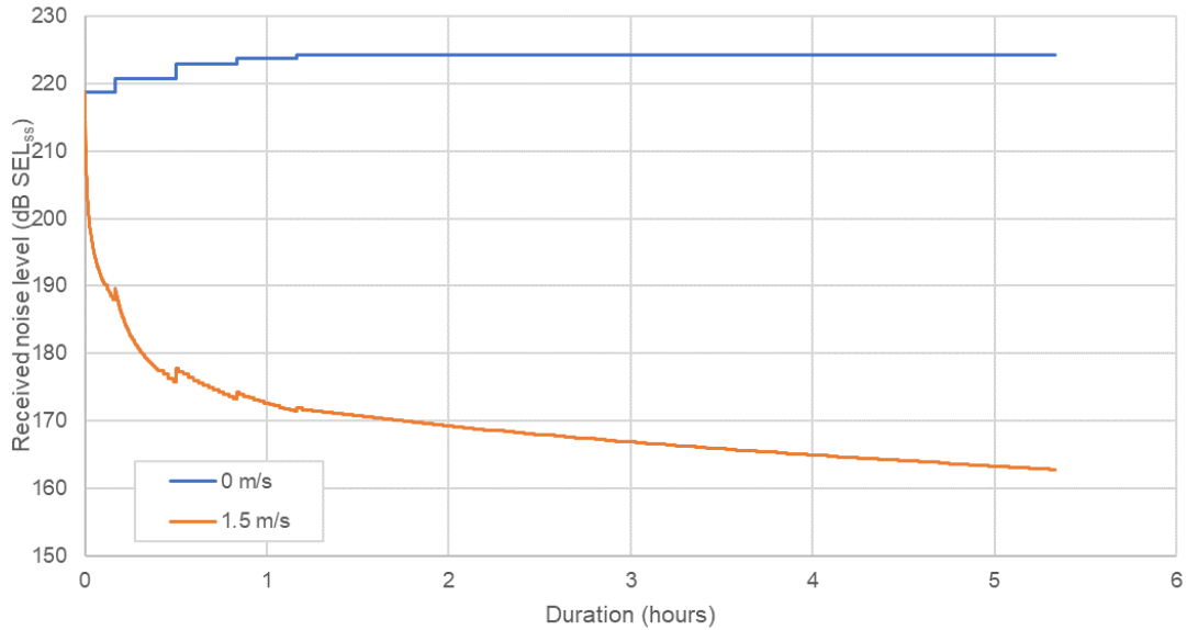
Figure 4-3 Received single-strike noise levels ( SEL_{ss} ) for receptors during the monopile foundation parameters at the Dogger Bank West: West location, assuming both a stationary and fleeing receptor starting at a location 1 m from the noise source
